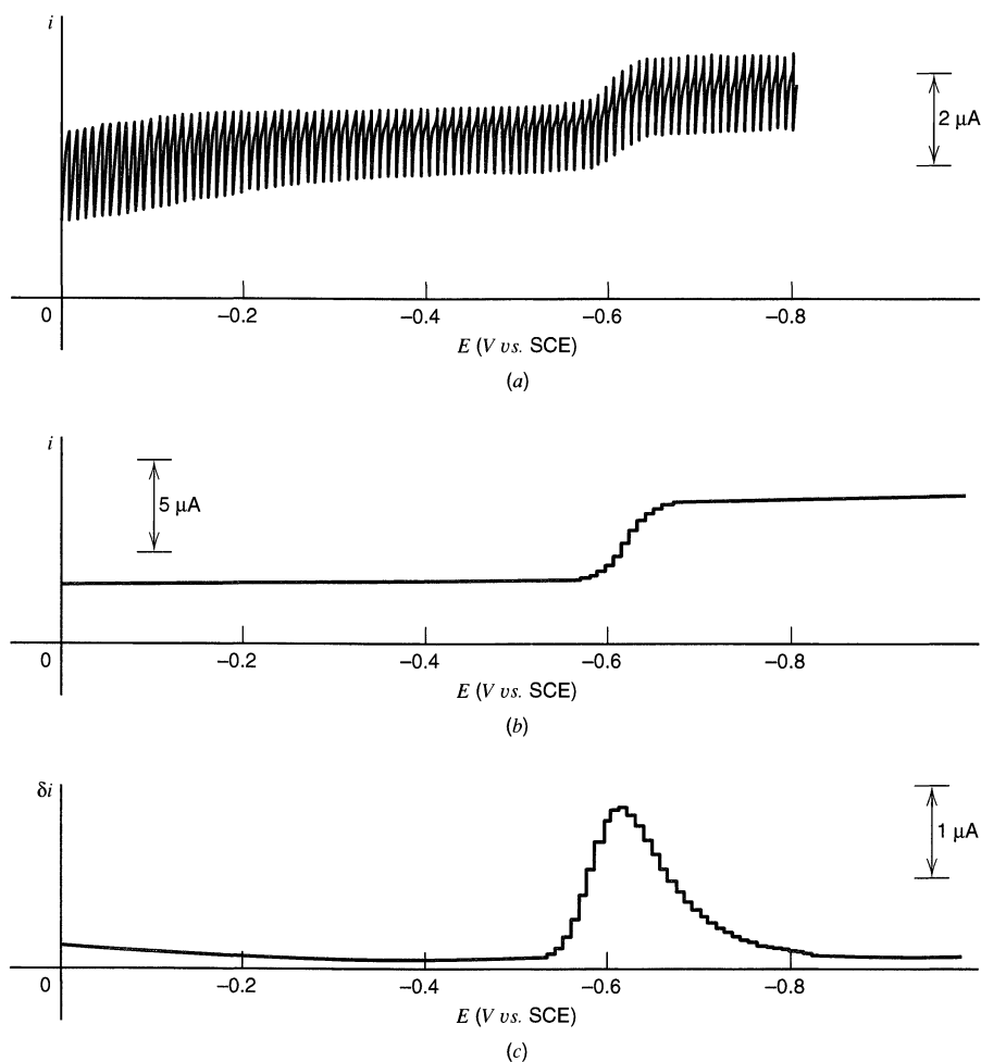
Figure 7.3.18 Polarograms at a DME of 10^{-3} M \text{Fe}^{3+} and 10^{-4} M \text{Cd}^{2+} in 0.1 M HCl. (a) Conventional dc mode. (b) Normal pulse mode, E_b = -0.2 V vs. SCE. (c) Differential pulse mode, \Delta E = -50 mV.
