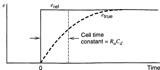
Figure 15.6.2 The effect of the cell time constant on the rise of the true working electrode potential after an instantaneous step is applied.
