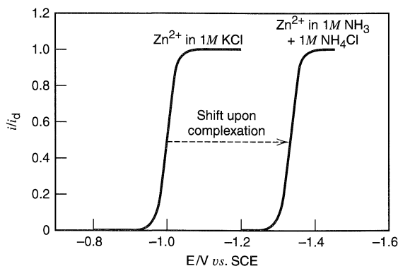
Figure 5.4.2 Shift of a reversible wave upon complexation of the reactant. Left curve is the reduction wave for Zn^{2+} in 1\text{ M KCl} at a Hg electrode ( E_{1/2} = -1.00\text{ V vs. SCE} ). Right curve is for Zn^{2+} in 1\text{ M NH}_3 + 1\text{ M NH}_4\text{Cl} ( E_{1/2} = -1.33\text{ V vs. SCE} ). Complexation by ammonia lowers the free energy of the oxidized form, so that it is no longer possible to reduce Zn(II) to the amalgam at the potentials of the wave recorded in the absence of ammonia. By applying a more negative potential, the combined free energy of Zn(II) plus the 2e on the electrode is elevated to match that of Zn(Hg) and interconversion between Zn(II) and Zn(Hg) becomes possible.
