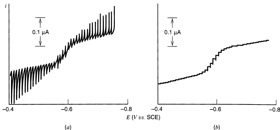
Figure 7.3.3 Polarograms at a DME for 10^{-5} M \text{Cd}^{2+} in 0.01 M \text{HCl} . (a) Conventional dc mode. (b) Tast mode. Note that the tast method eliminates the sharp nonfaradaic spikes appearing at each drop fall. The PZC is near -0.5 \text{ V} in this experiment, hence the charging current spikes appear “anodic” at more positive potentials and “cathodic” at more negative ones.
