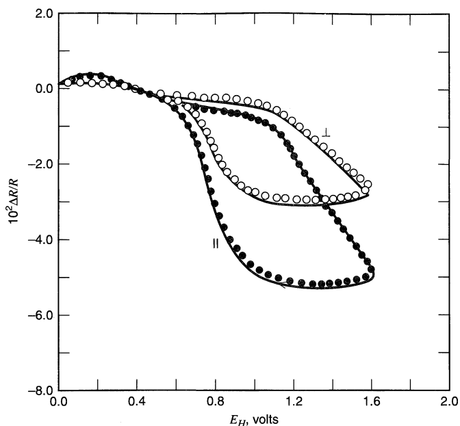
Figure 17.1.12 Reflectance change vs. potential for a platinum electrode in 1.0 M HClO 4 . v = 30 mV/s. Separate data are shown for parallel and perpendicular polarization. The curves are for Ar-saturated solutions, and the points are for O 2 -saturated solutions. Note that the reflectance changes are independent of the faradaic reduction of O 2 , which takes place in the negative part of this range. [From J. D. E. McIntyre and D. M. Kolb, Symp. Faraday Soc. , 4, 99 (1970), with permission.]
