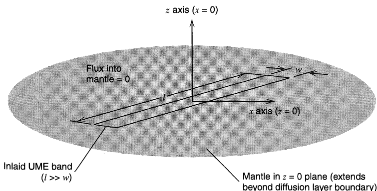
Figure 5.3.3 Diffusional geometry at a band electrode. Normally the length of the electrode is very much larger than the width, and the three-dimensional diffusion at the ends does not appreciably violate the assumption that diffusion occurs only along the x and z axes.
