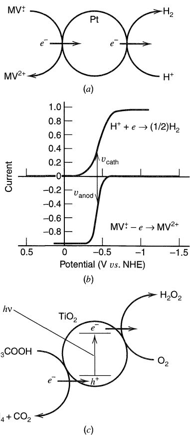
Figure 18.2.11 (a) Schematic representation of the two half-reactions occurring at a Pt particle that catalyzes the overall reaction MV^{\cdot+} + H^+ \rightarrow MV^{2+} + (1/2)H_2 . (b) Current-potential curves for the two half reactions. Arrows show predicted currents and the mixed potential where v_{cath} = v_{anod} (or i_c = i_a ). (c) Half-reactions occurring during irradiation of a TiO_2 particle in an oxygen-saturated acetic acid solution.
