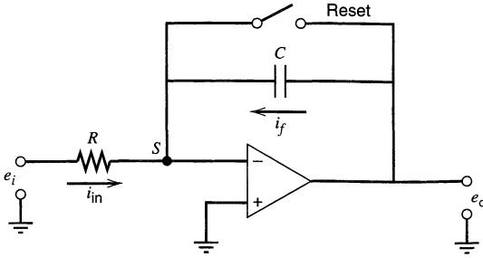
Figure 15.2.5 A voltage integrator.
