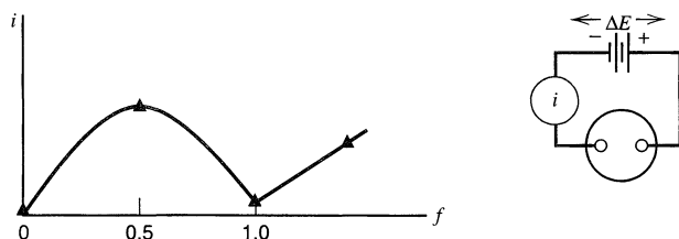
Figure 11.5.6 Two-electrode amperometric titration of \text{Fe}^{2+} with \text{Ce}^{4+} with a constant potential difference, \Delta E , impressed between two platinum indicator electrodes (see Figure 11.5.4).
