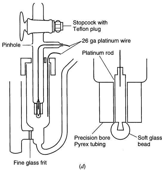
Figure 11.7.1 Continued (c) Close-up of electrode portion for single-electrode configuration of (b). (d) Capillary-wire single-electrode thin-layer electrode.
