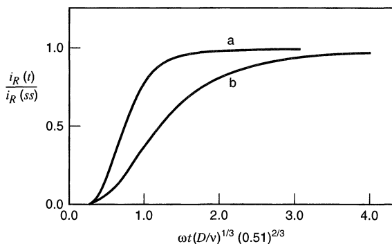
Figure 9.5.2 Simulated ring-current transients. Curve a : Potential step at the disk. Curve b : Current step at the disk. [From K. B. Prater and A. J. Bard, J. Electrochem. Soc. , 117 , 207 (1970), with permission of the publisher, The Electrochemical Society, Inc.]
