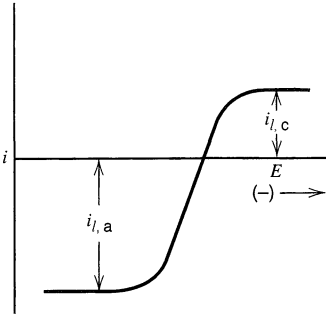
Figure 1.4.3 Current-potential curve for a Nernstian system involving two soluble species with both forms initially present.
