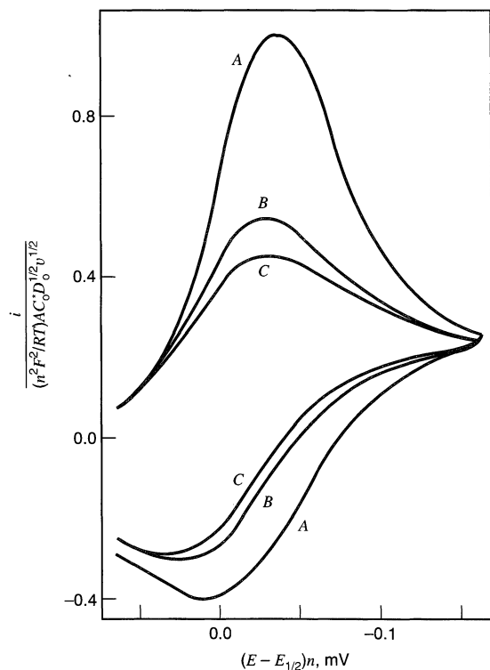
Figure 14.3.10 Effect of scan rate on cyclic voltammograms when the reactant is weakly adsorbed. Calculated for \beta_O C_O^* = 0.01 and 4\Gamma_{O,s} \beta_O v^{1/2} (nF/RT)^{1/2} / (\pi D_O)^{1/2} values of: curve A, 5.0; curve B, 1.0; curve C, 0.1. (Curve C corresponds to an essentially unperturbed reaction). Note that relative scan rates are 2500:100:1. [Reprinted with permission from R. H. Wopschall and I. Shain, Anal. Chem. , 39 , 1514 (1967). Copyright 1967, American Chemical Society.]
