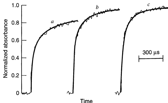
Figure 17.1.18 Transient absorbances caused by potential steps of 800- \mu\text{s} width from 0.40 to 0.80 V vs. SCE. Pulses were repeated at 30 Hz for 2 min, and transients were averaged. Curve a : 0.182 mM TAA in acetonitrile. Curve b : 0.182 mM TAA and 0.182 mM AF. Curve c : 0.167 mM TAA and 0.333 mM AF. Solid curves are fitted results yielding the rate constant given in the text. [Reprinted with permission from N. Winograd and T. Kuwana, J. Am. Chem. Soc. , 93 , 4343 (1971). Copyright 1971, American Chemical Society.]
