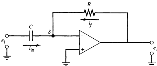
Figure 15.2.6 A differentiator.
