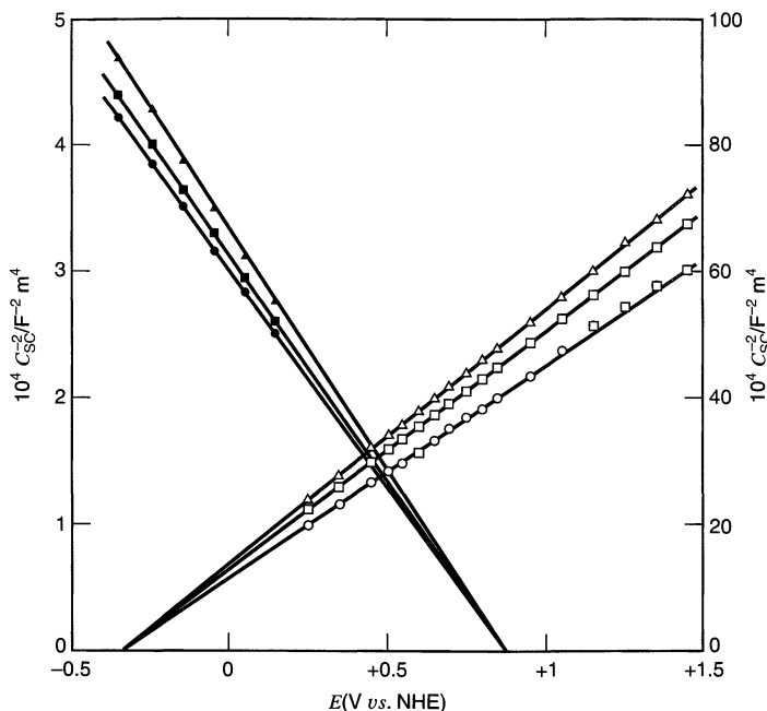
Figure 18.5.2 Mott-Schottky plots for n - and p -type InP, (111) face. Electrolyte composition: 1 M KCl + 0.01 M HCl, n -type: (○) 200 Hz, (□) 2500 Hz, (Δ) 20,000 Hz; p -type: (●) 200 Hz, (■) 2500 Hz, (▲) 20,000 Hz. The vertical axis to the left applies to p -type, the one to the right to n -type. [From A. M. Van Wezemaal, W. H. Laftere, F. Cardon, and W. P. Gomes, J. Electroanal. Chem. , 87 , 105 (1978), with permission.]
