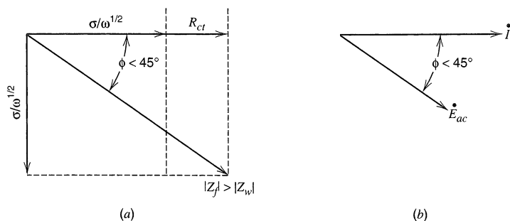
Figure 10.3.3 (a) Vector diagram showing the effect of R_{ct} on the impedance. (b) Phase relationship between I and E for a system with significant R_{ct} .
