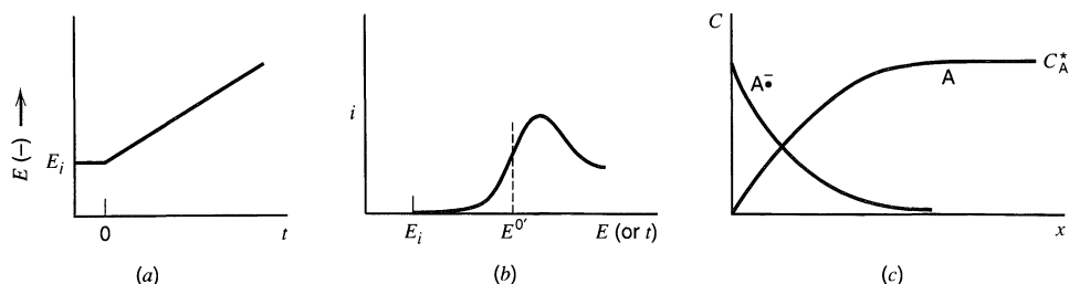
Figure 6.1.2 (a) Linear potential sweep or ramp starting at E_i . (b) Resulting i - E curve. (c) Concentration profiles of A and A^- for potentials beyond the peak.
