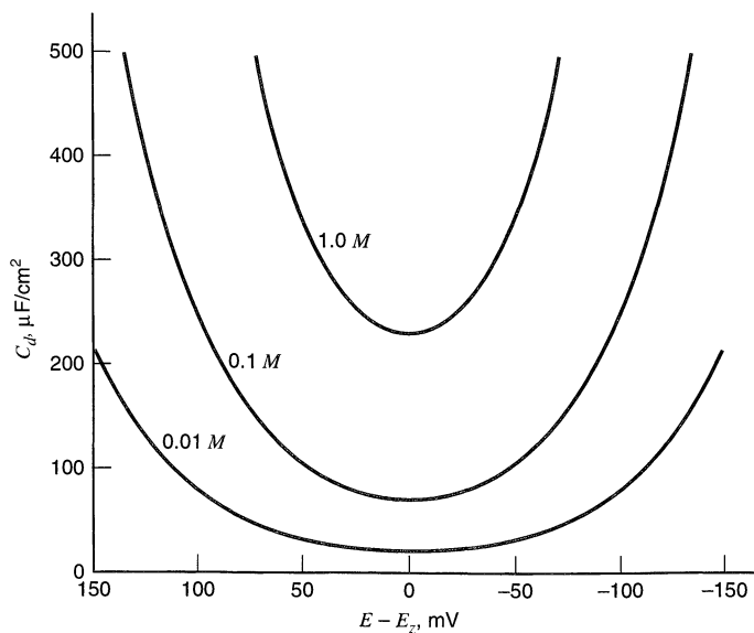
Figure 13.3.5 Predicted differential capacitances from the Gouy–Chapman theory. Calculated from (13.3.21) for the indicated concentrations of a 1 : 1 electrolyte in water at 25°C. Note the very restricted potential scale. The predicted capacitance rises very rapidly at more extreme potentials relative to E_z .
